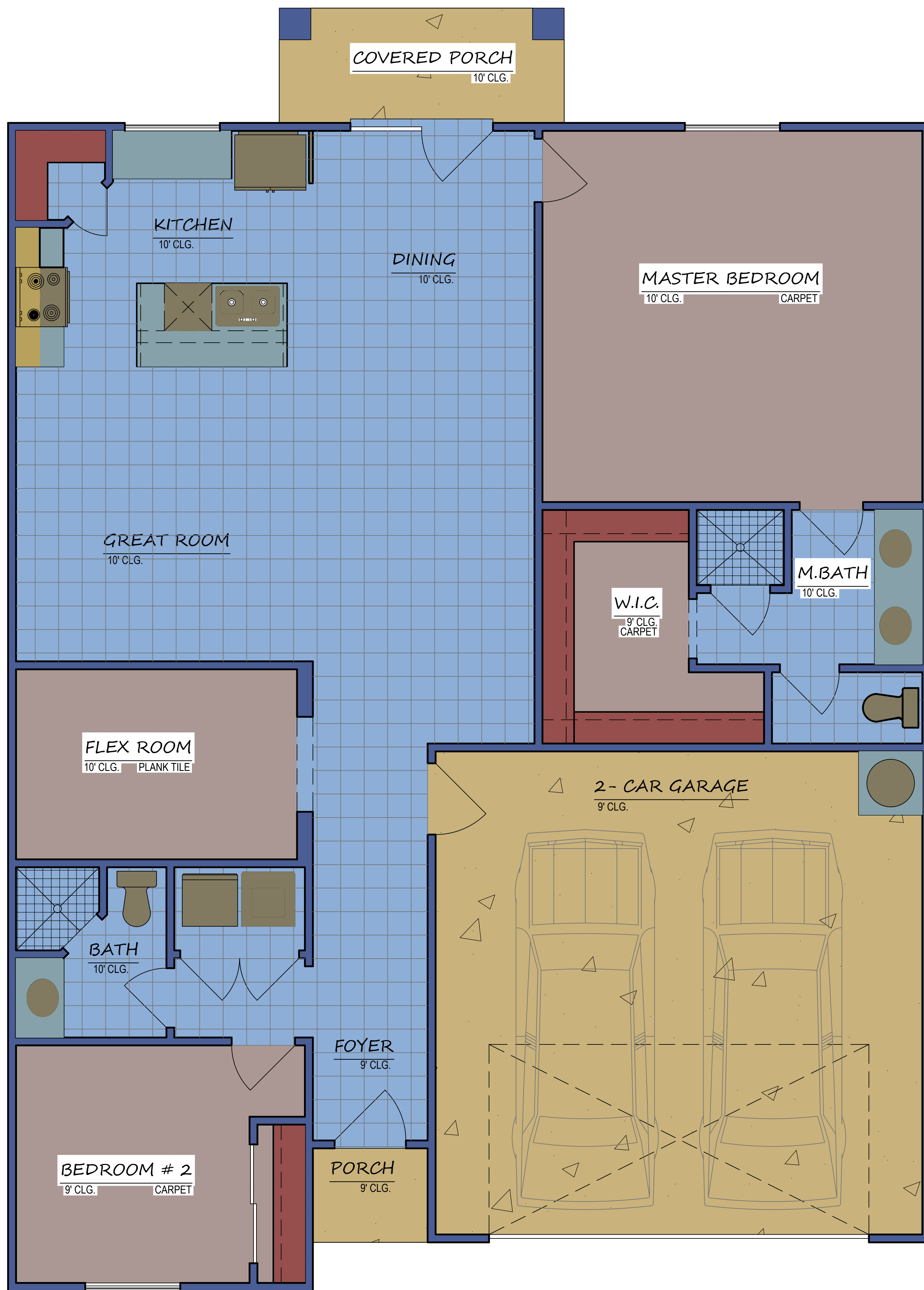
FLOOR PLAN THE "GRANADA"
